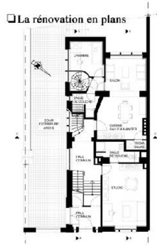
PLAN REZ-DE-CHUSSEE
